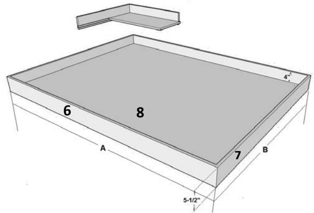
Cut List for Pedestal and Platform Parts.
