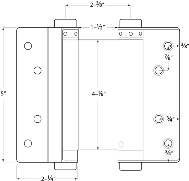
OPEN POSITION
