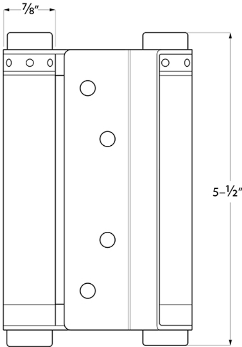
CLOSED POSITION
